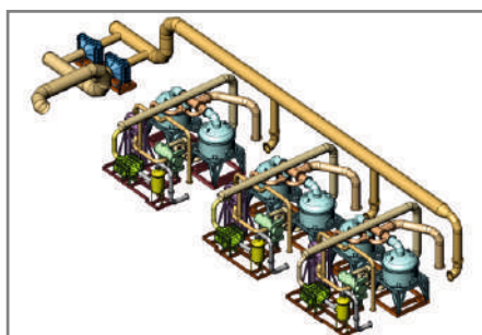
NPCIL - TAPP 3 & 4 Dual Fixed Bed type
